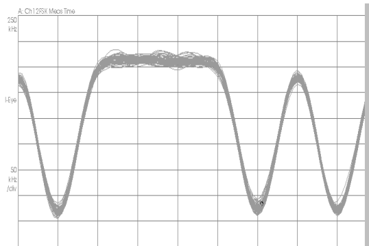
Figure 3. Modulation
