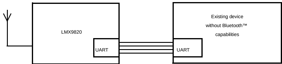
Figure 17. Bluetooth Functionality
