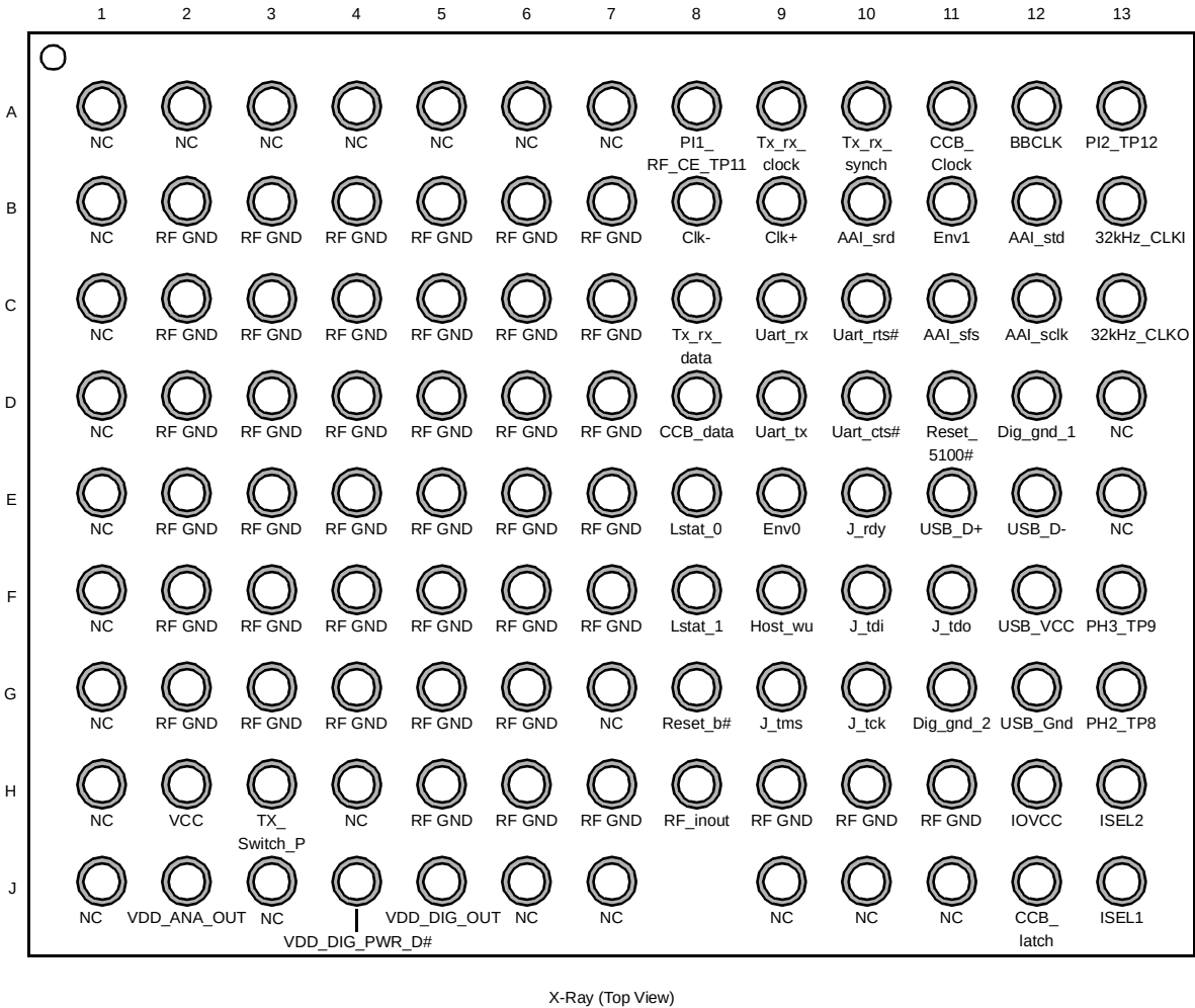
Figure 2. Connection Diagram LMX9820
